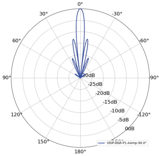
Port 1
